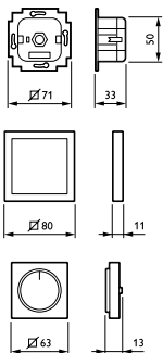
UID8620/00 DALI Dimmer
